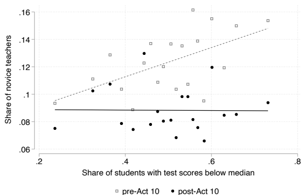
Figure 3: Vertical Sorting
